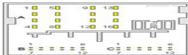
40 (16+12+12) pin QuadLock Fakra Head Unit / Car Stereo connector
