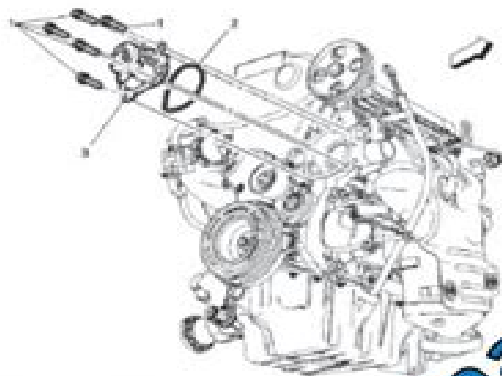
Fig. 74: Water Pump (2H0) Courtesy of GENERAL MOTORS COMPANY
