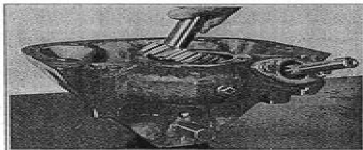
Figure 8-27 Removing Sector
