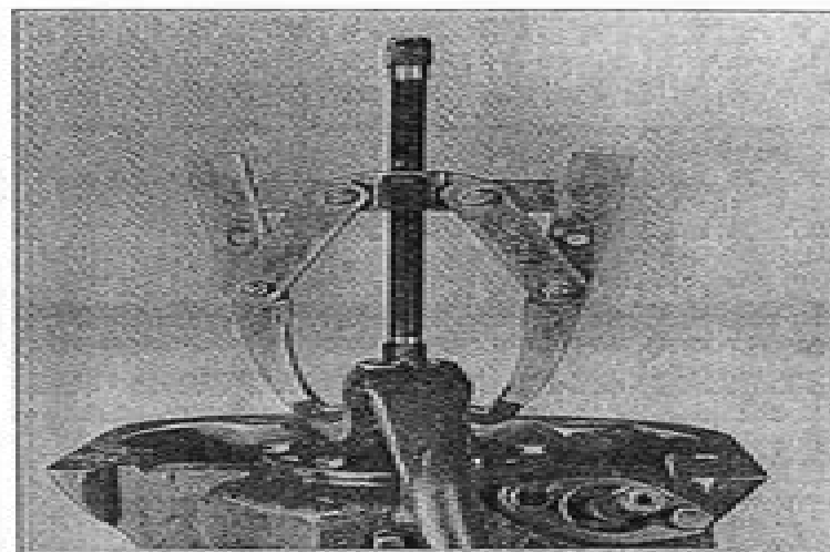
Figure 8-26 Removing Steering Arm
