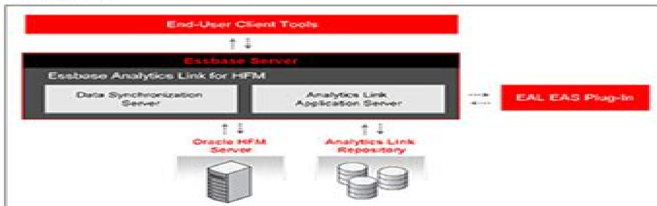
Figure 8 - Essbase Analytics Link Functional Architecture
