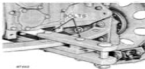
Drawbar in Short Position
