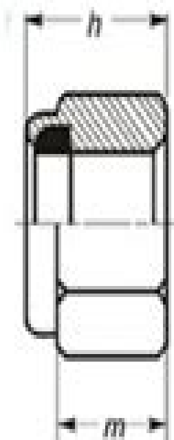
DIN 985 DIN 982 Nylon Lock Nuts Prevailing Torque Type Hexagon Thin Nuts With Nylon Insert
