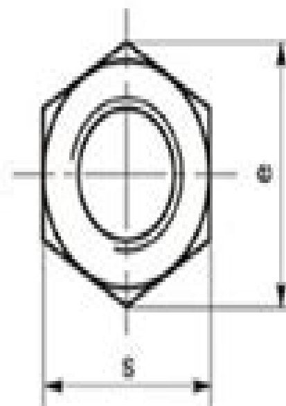
DIN 985 DIN 982 Nylon Lock Nuts Prevailing Torque Type Hexagon Thin Nuts With Nylon Insert
