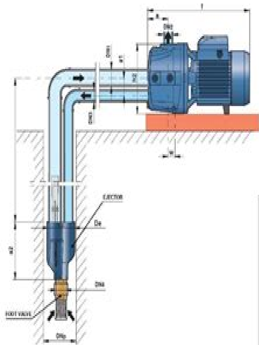
JET PUMP
