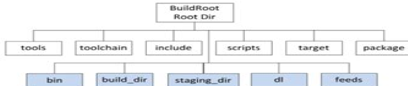
Figure 1. OpenWrt Buildroot Source Tree (The folders in the second lines are generated during compilation).
