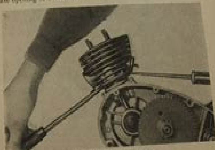
Fig. 2. Removing the Cylinder
