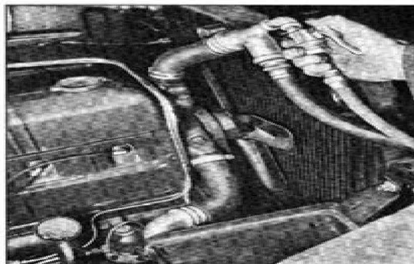
Fig. 122—Reverse Flushing Block and Head
