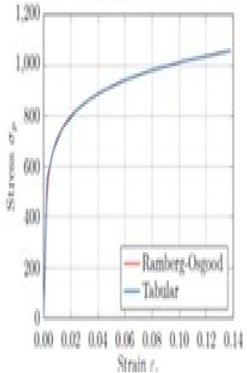
Stress-Strain-Curve
