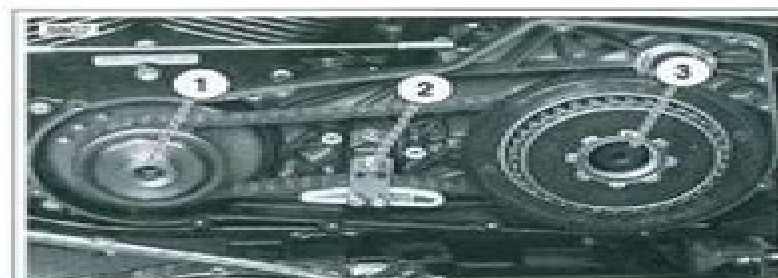
Figure 6-6. Compensating Sprocket and Clutch Hub
