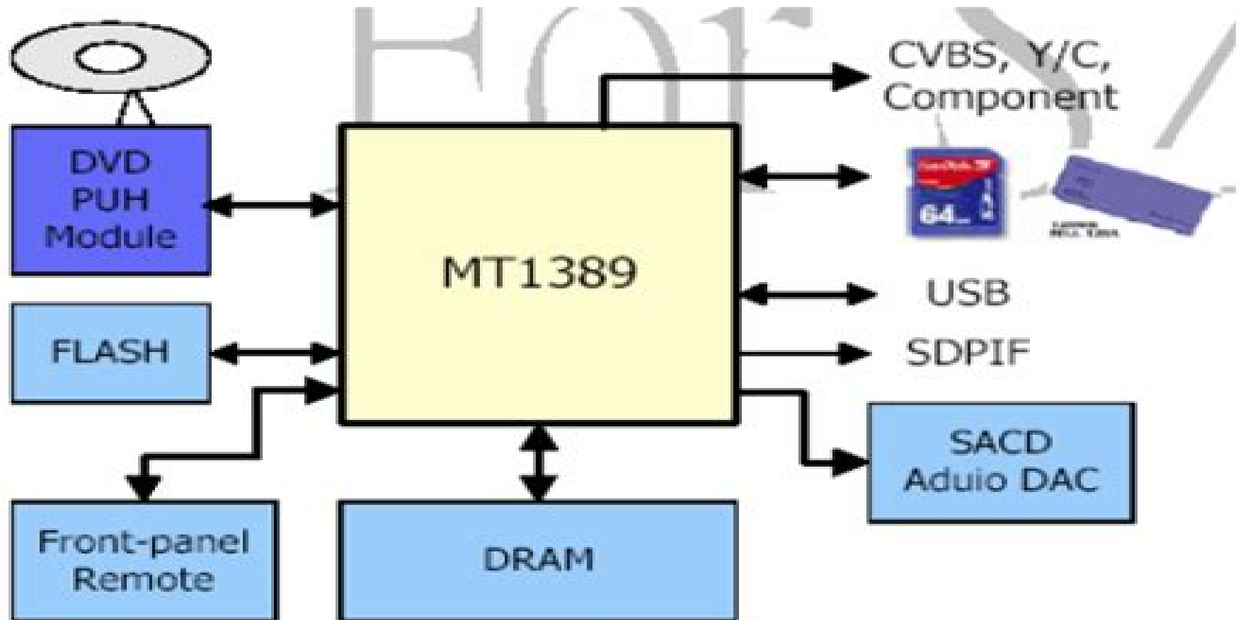
DVD Player System Diagram Using MT1389
