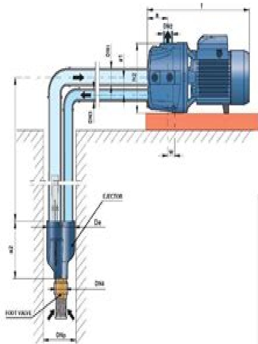
JET PUMP
