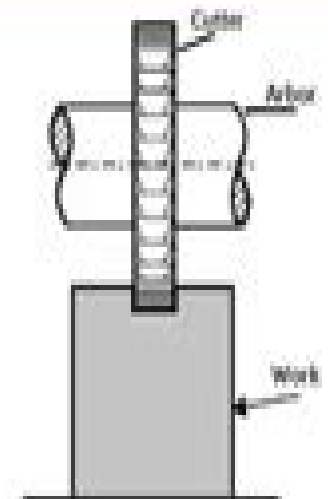
Keyway Milling Operation
