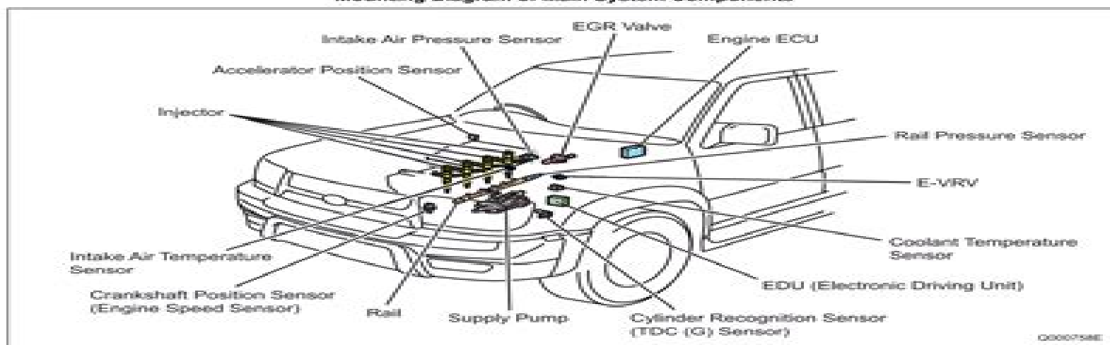
Mounting Diagram of Main System Components
