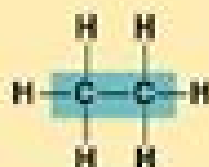
Ethane
