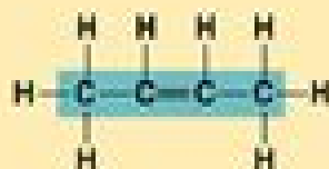
2-Butene
