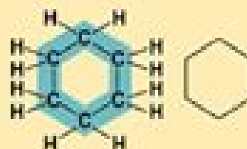
Cyclohexane
