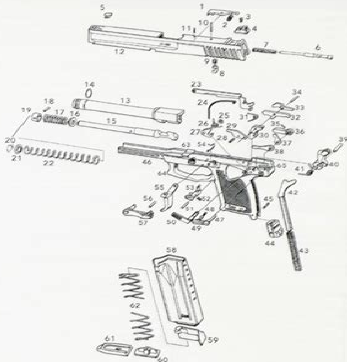
Figure 15 Mark 23 / MK23 Exploded Diagram
