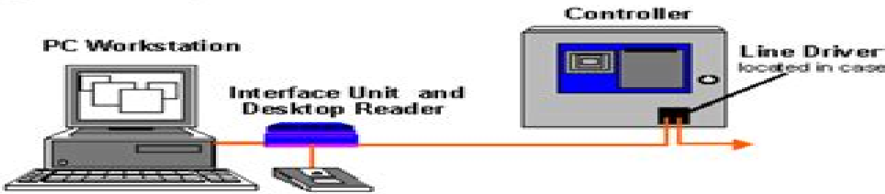
Figure 2. Desktop Reader Only (Multi-PC System)
