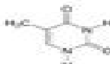
Thymine
