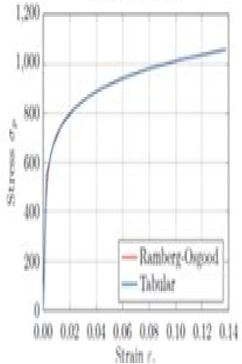
Stress-Strain-Curve
