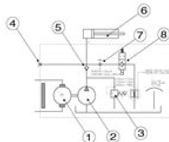
Figure 5.1 Hydraulic system (D450 1104)
