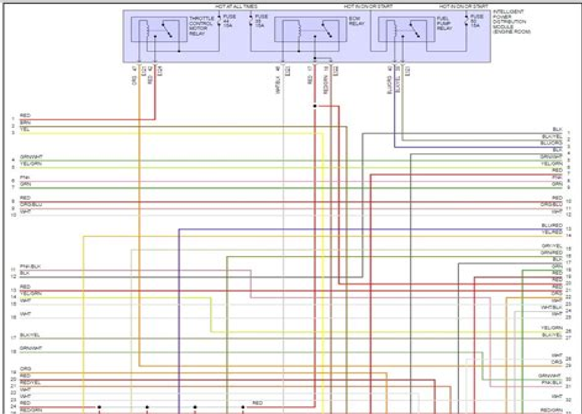
Fig 2: 2.5L, Engine Performance Circuit (2 of 4)
