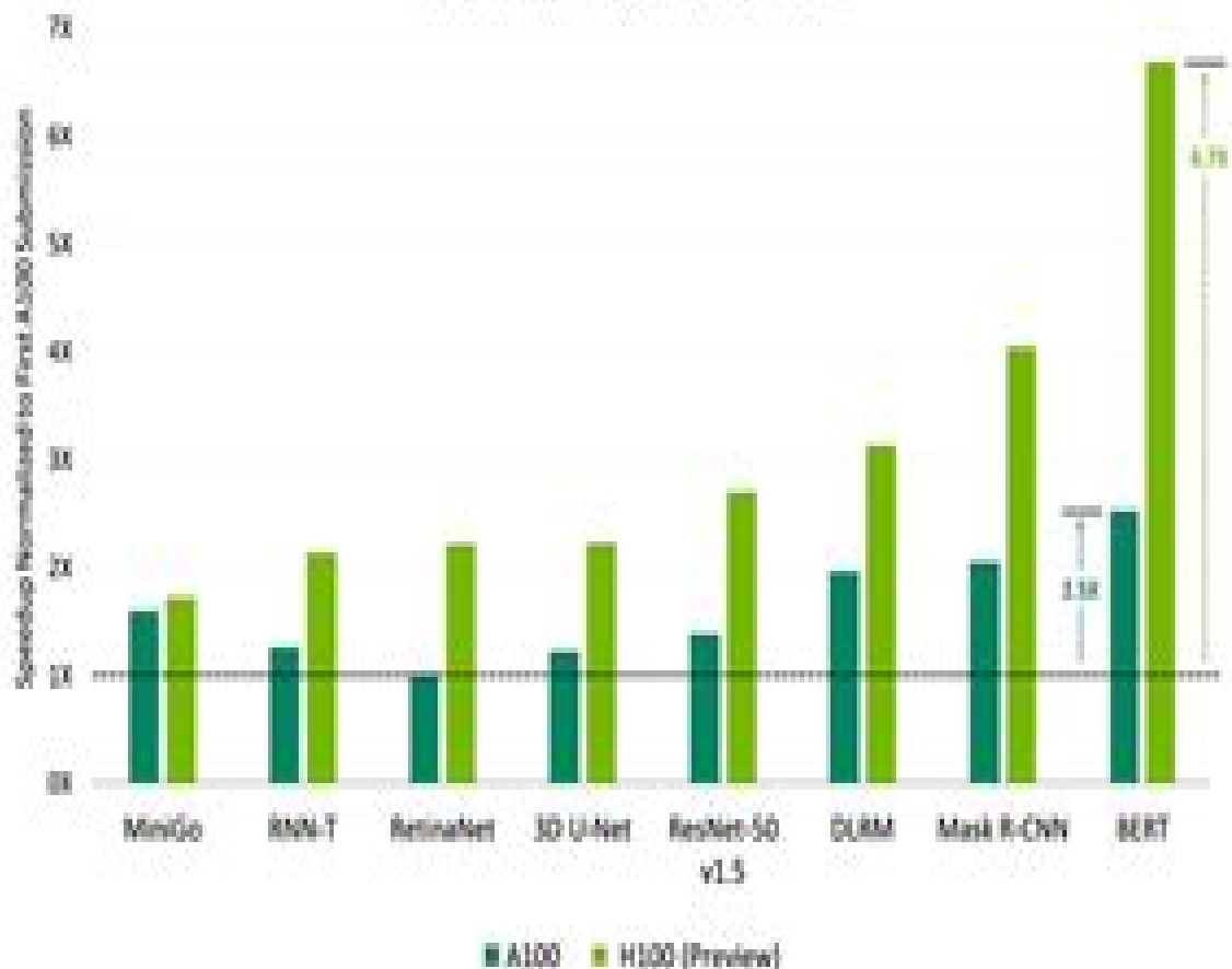
MLPerf™ Training v2.1 Performance
