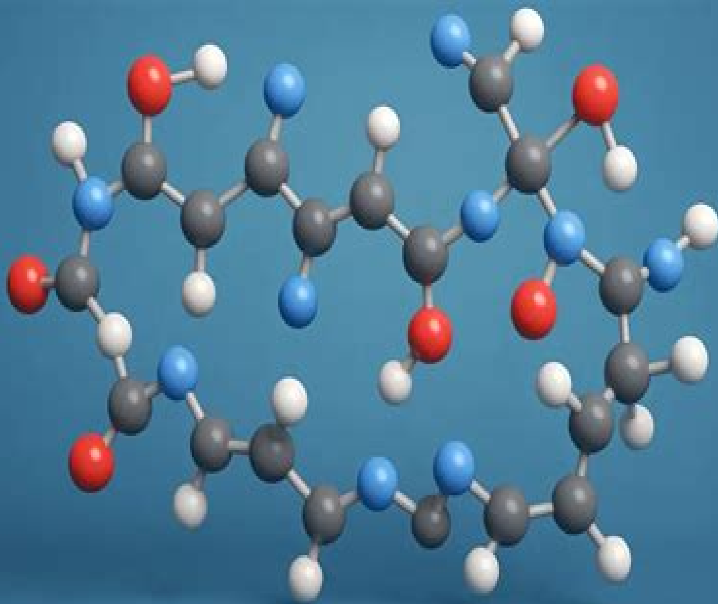
SUBSTANCE P
