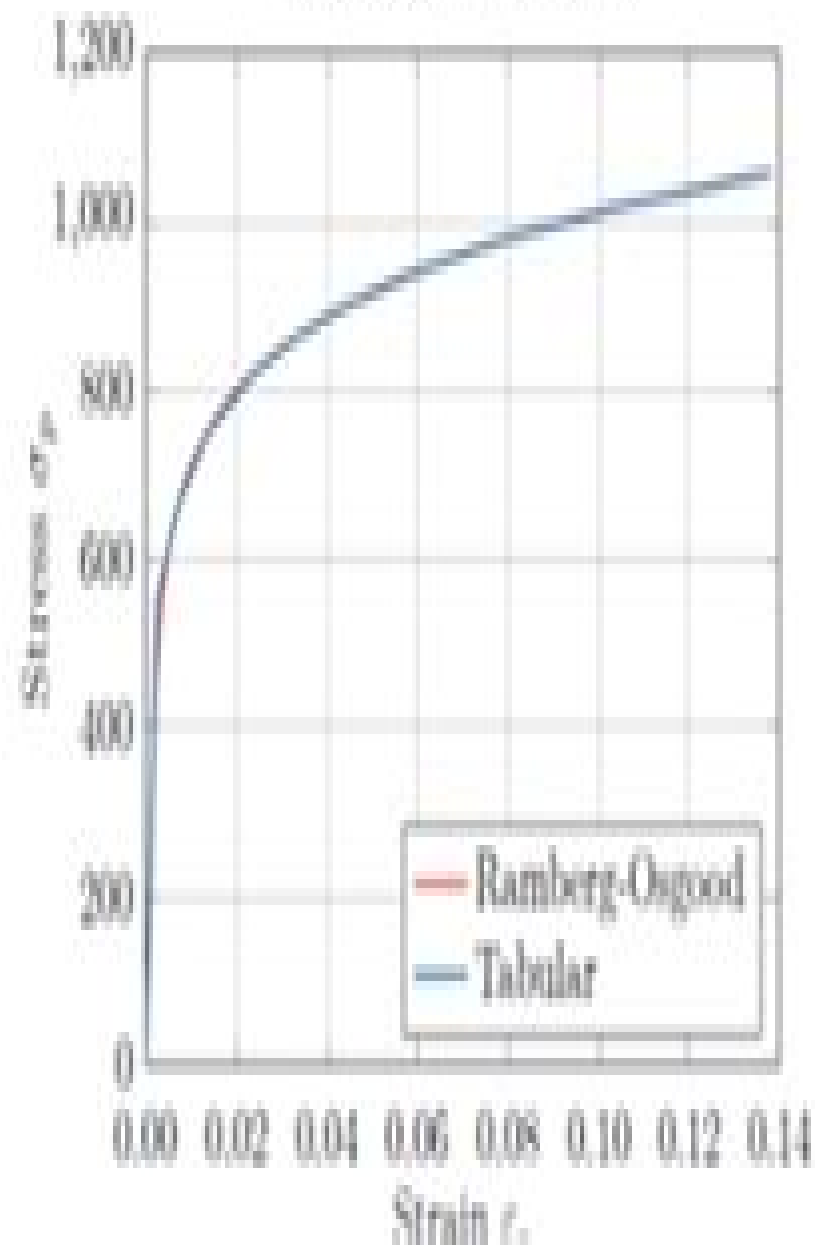
Stress-Strain-Curve
