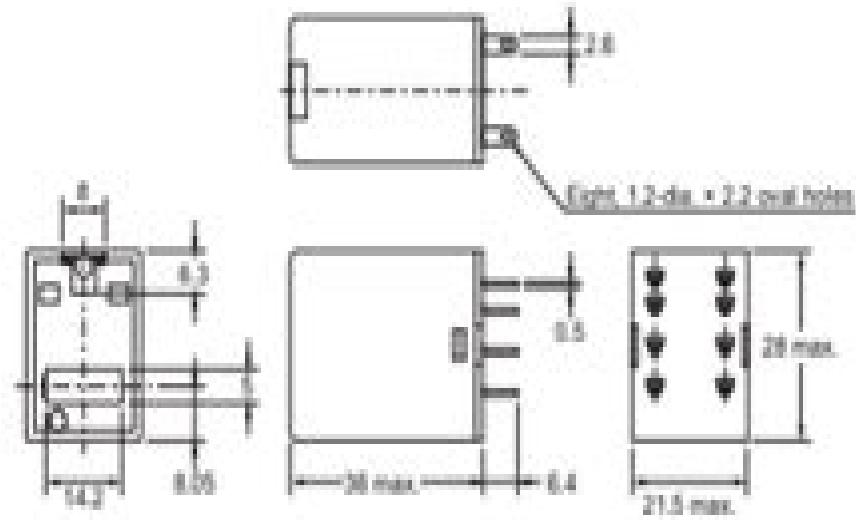
Terminal Arrangement/Internal Connections (Bottom View)
