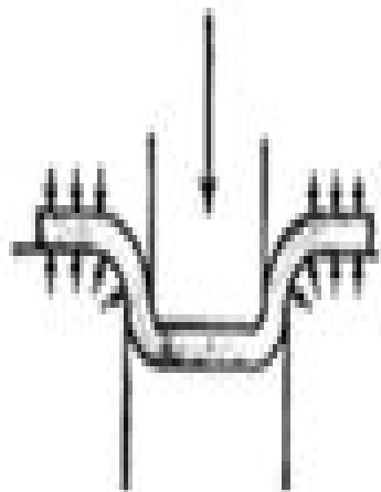
Deep Drawing
