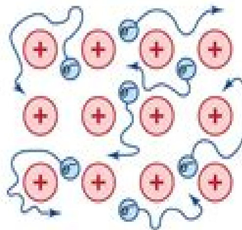
metallic bond
