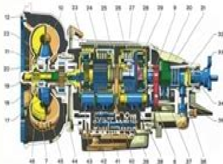
3-speed transmission with torque converter
