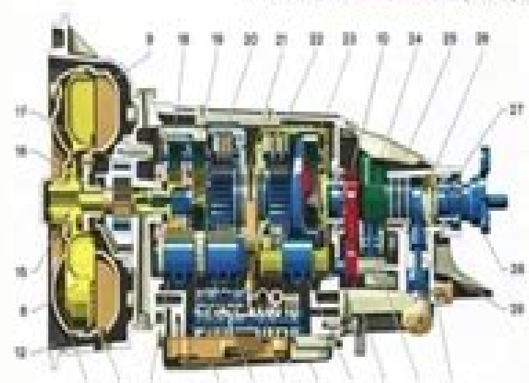
4-speed transmission with fluid coupling
