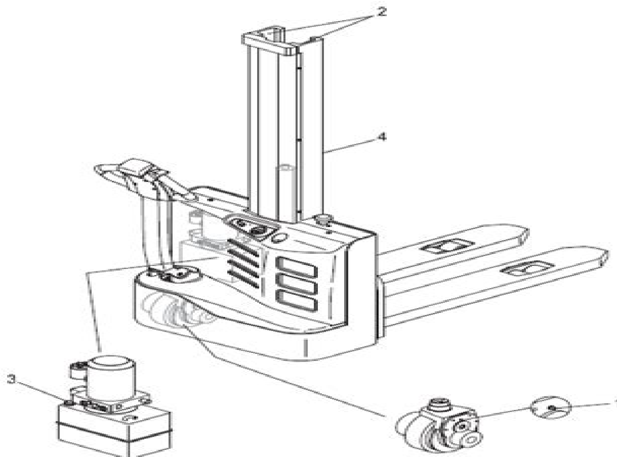
Figure 3-4 Lubrication Diagram
