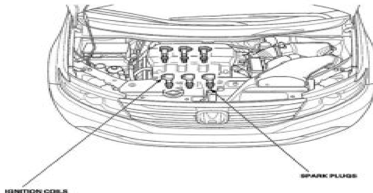
Fig. 1: Identifying Ignition System Replacement Components Courtesy of AMERICAN HONDA MOTOR CO., INC.
