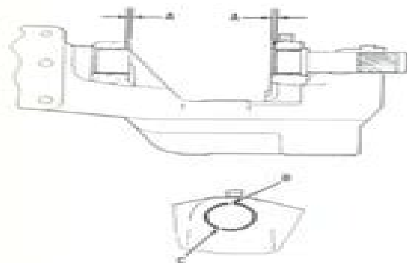
Fig. 9—Axle pivot bushings should be installed as shown for 362 model. Note (B) should be aligned with grease passage and shim (C) should be in position indicated.
