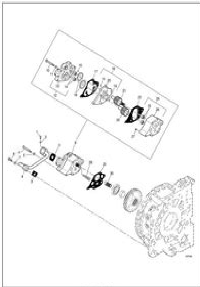
Figure 08. Oil Pump
