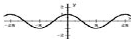
f(x) = \cos x Trigonometric Functions
