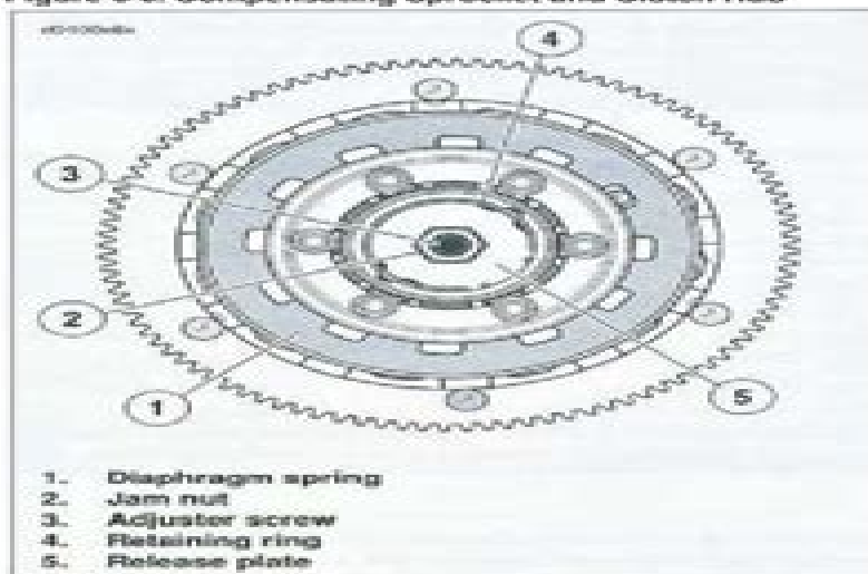
Figure 6-7. Clutch
