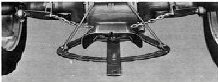
Fig. 9 - Swinging Drawbar with PTO Adapter Installed
