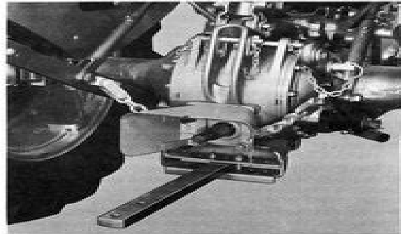
Fig. 8 - Universal Drawbar with PTO Adapter Installed
