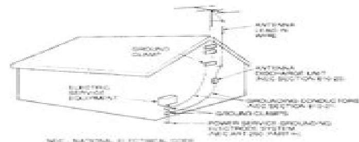
FIGURE 73.1: EXAMPLE OF ANTENNA GROUNDING AS PER NATIONAL ELECTRICAL CODE
