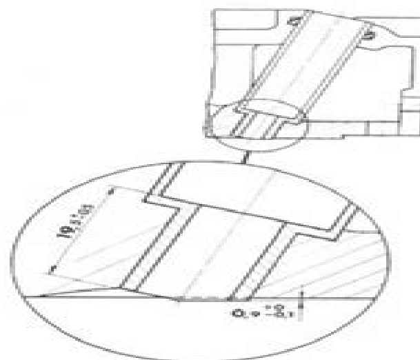
Fig. 9. Adjusting the injector sleeve.
