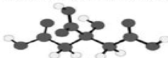
Citric acid
