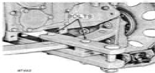
Drawbar in Short Position
