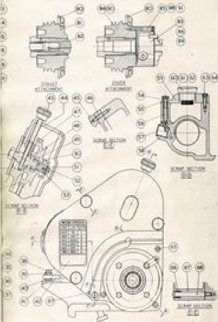
WORKHEAD
