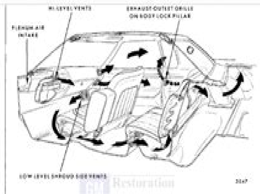
Fig. 4-Body Ventilation Flow Pattern - Cadillac "F" Body Styles, Buick Wildcat, Chevrolet "F", and Oldsmobile Toronado
