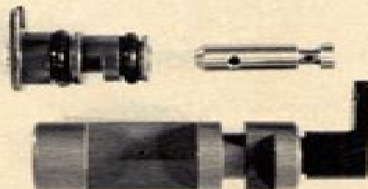
Carburetor metering valve assembly and throttle vane. Small hole in center feeds fuel into airstream. Two additional holes (not pictured) at end of vane cut-out, do likewise.
