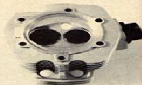
Combustion chamber, intake valve considerably larger than exhaust valve. Note glow plug hole offset towards exhaust.
