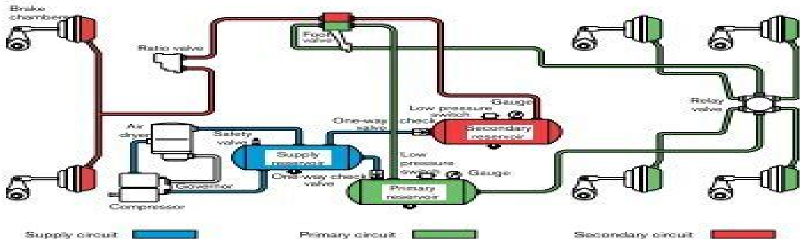
Figure 29. Simple dual circuit with brakes applied.
