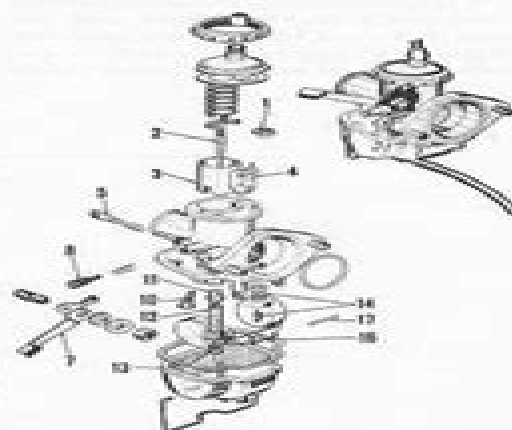
Fig. HN2-3—Exploded view of side draft carburetor typical of that used on 50 and 55 cc Sport Cub models.
