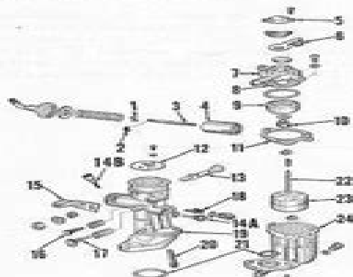
Fig. HN2-1—Exploded view of typical carburetor used on 50 and 55 cc Super Cub and Trail Cub models. Type A carburetors have idle jet at 14A. Type B & C carburetors have idle jet located at 14B.
