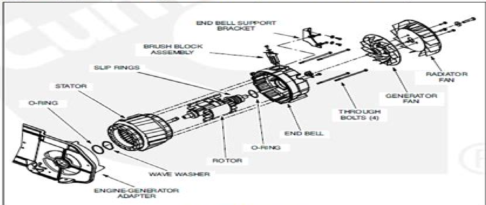
FIGURE 6-1. GENERATOR
