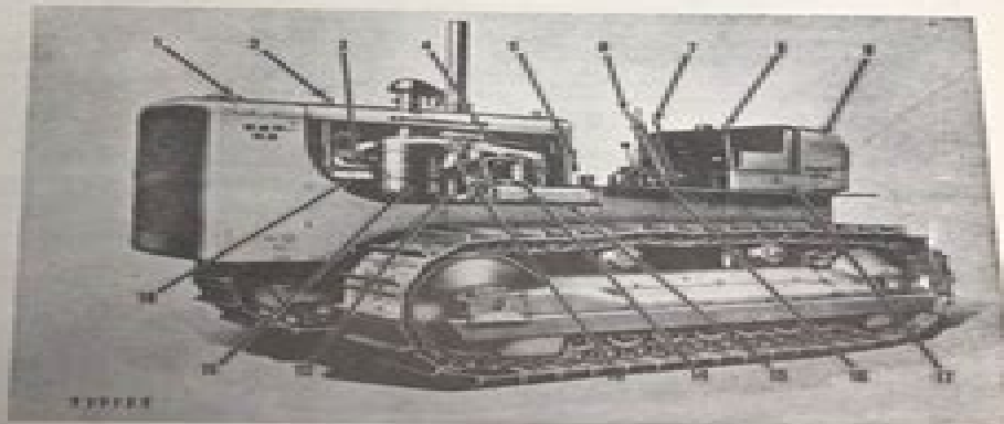
D8 TRACTOR - LEFT FRONT VIEW
