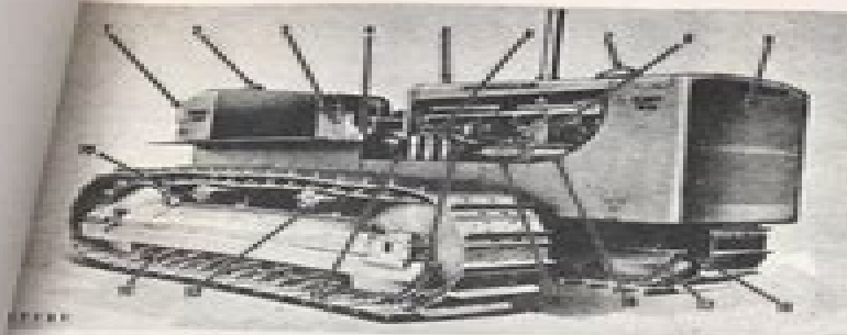
D8 TRACTOR - RIGHT FRONT VIEW
