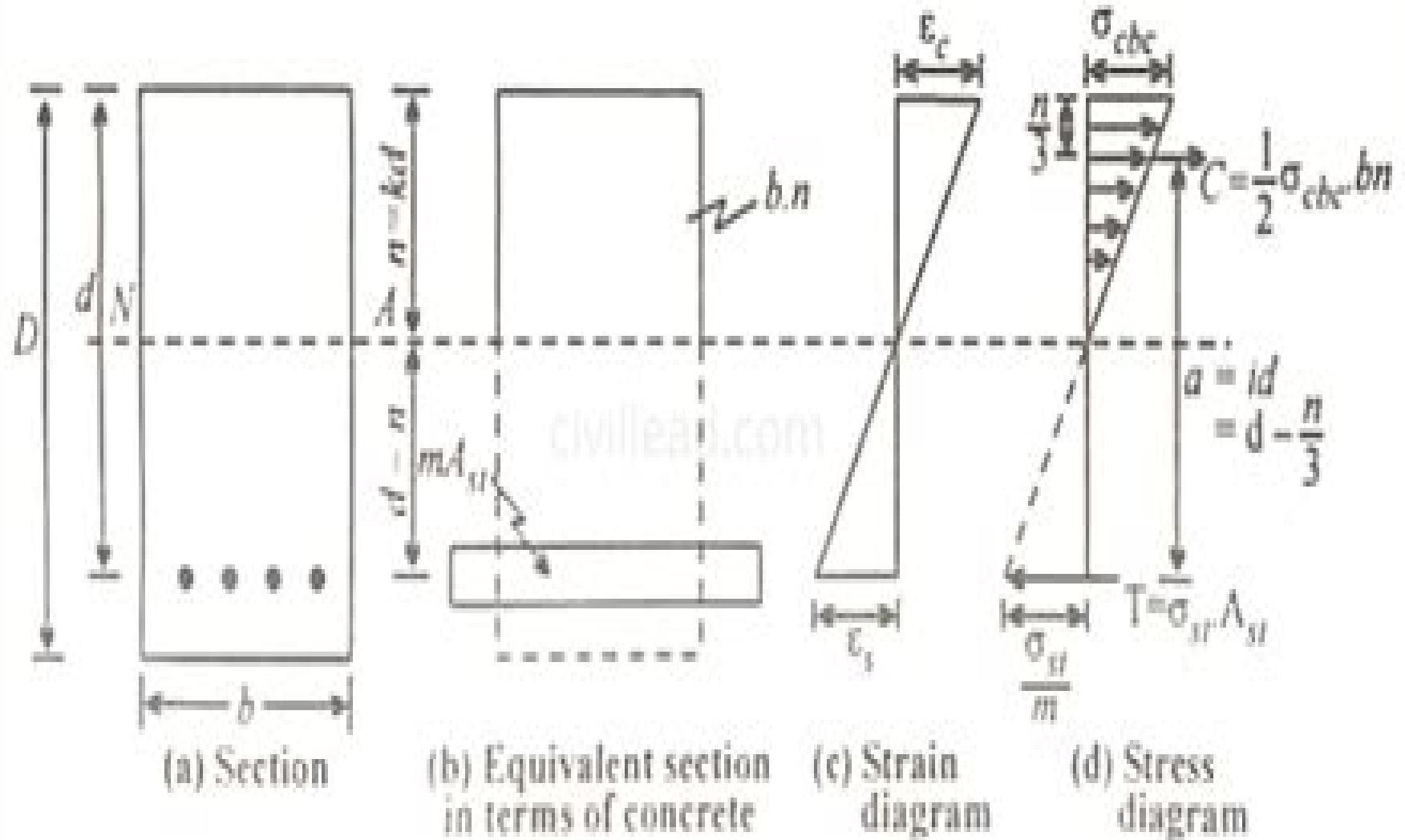
Singly Reinforced Beam
