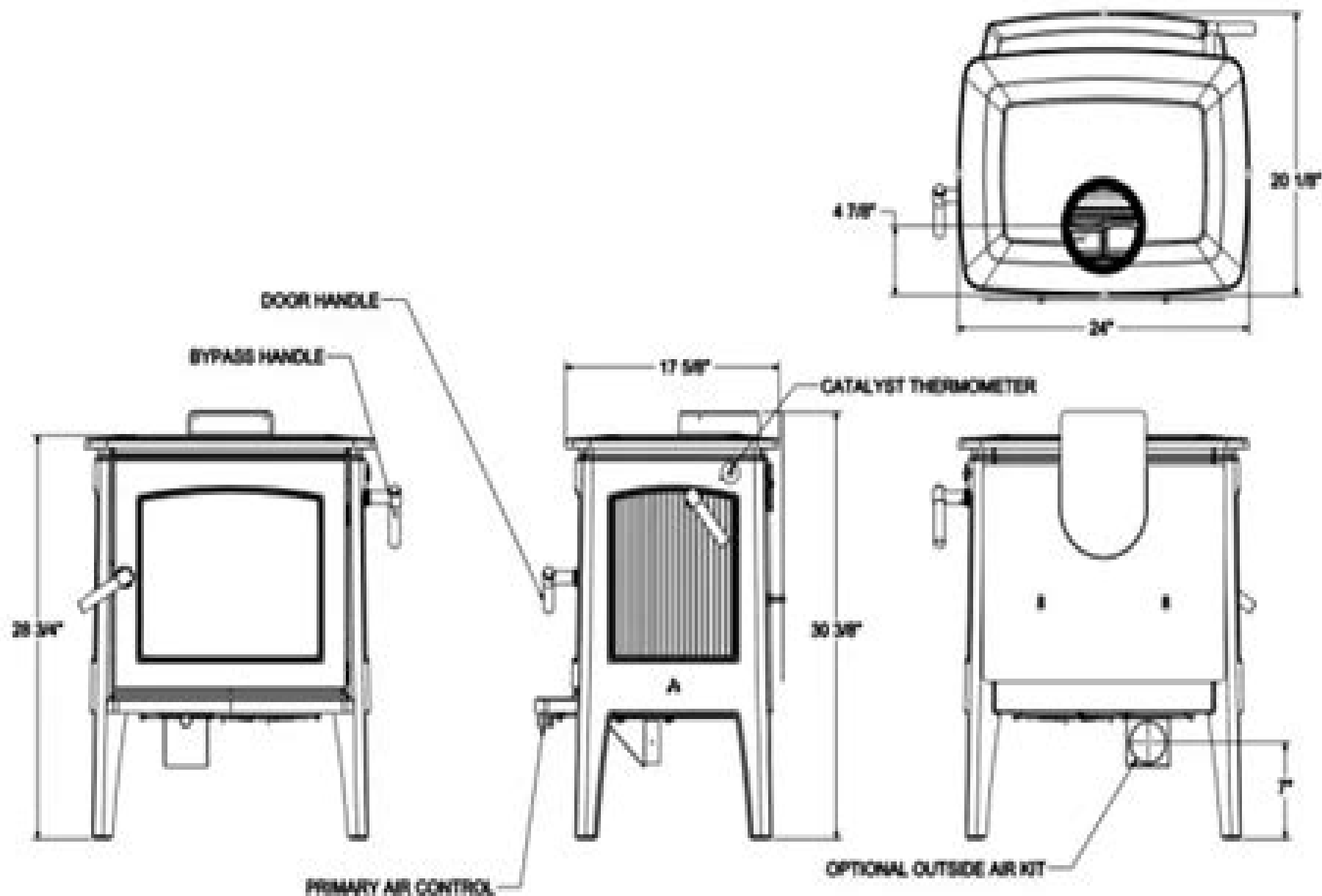
Figure 1 – Hipster 14 Dimensions
